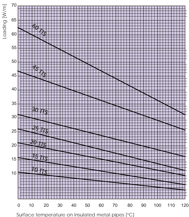
Temperature/Loading diagram TTS
